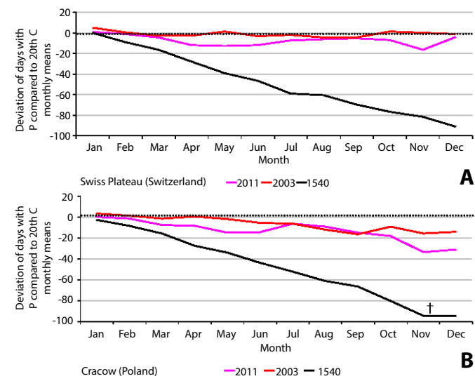
FIGURE 5.5 Cumulative deviations of the number of precipitation days in 1540 in Northern Switzerland and in Cracow (Poland) in comparison with twentieth century values
