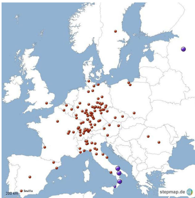
FIGURE 5.2 Spatial dimension of the extreme drought in 1540
