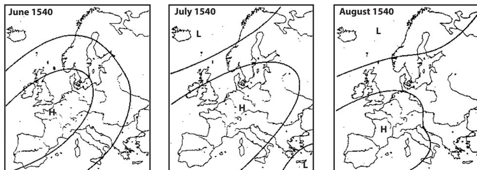
FIGURE 5.4 Reconstructed monthly surface pressure patterns for 1540
