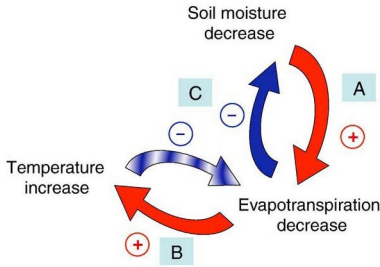
FIGURE 5.1 Processes contributing to soil moisture–temperature coupling and feedback loop
