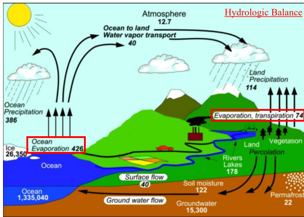
Units: Thousand cubic km for storage, and thousand cubic km/yr for exchanges Figure 8
