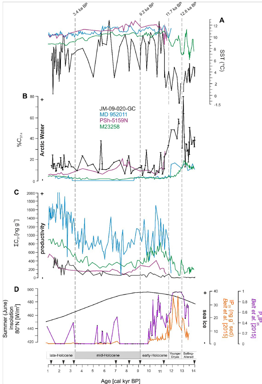
Fig. 4. Comparison of A) U_{37}^{K_e} -based sea surface temperatures (SSTs; right scale); B) \%C_{37:4} ; C) total alkenone concentrations ( \Sigma C_{37} ; ng\ g^{-1} ) from the current study (JM09-020 GC; black line), western Barents Sea (Martrat et al., 2003) (M23258; green line), the southwestern Barents Sea (Risebrobakken et al., 2010) (PSh-5159N; purple line), and the north-eastern Norwegian Sea (Calvo et al., 2002) (MD95-2011; blue line); and D) summer insolation (June) at 80°N (Berger and Loutre, 1991; black line, left scale) and IP_{25} (orange line, right scale), and P_{IP_{25}} (purple line, right scale) records from the core JM09-KA11 obtained from the western Barents Sea (after Belt et al., 2015) showing the sea ice conditions. The black triangles on the x axis denote the AMS ^{14}C converted to calibrated radiocarbon ages (after Łącka et al., 2015b). (For interpretation of the references to color in this figure legend, the reader is referred to the Web version of this article.)
