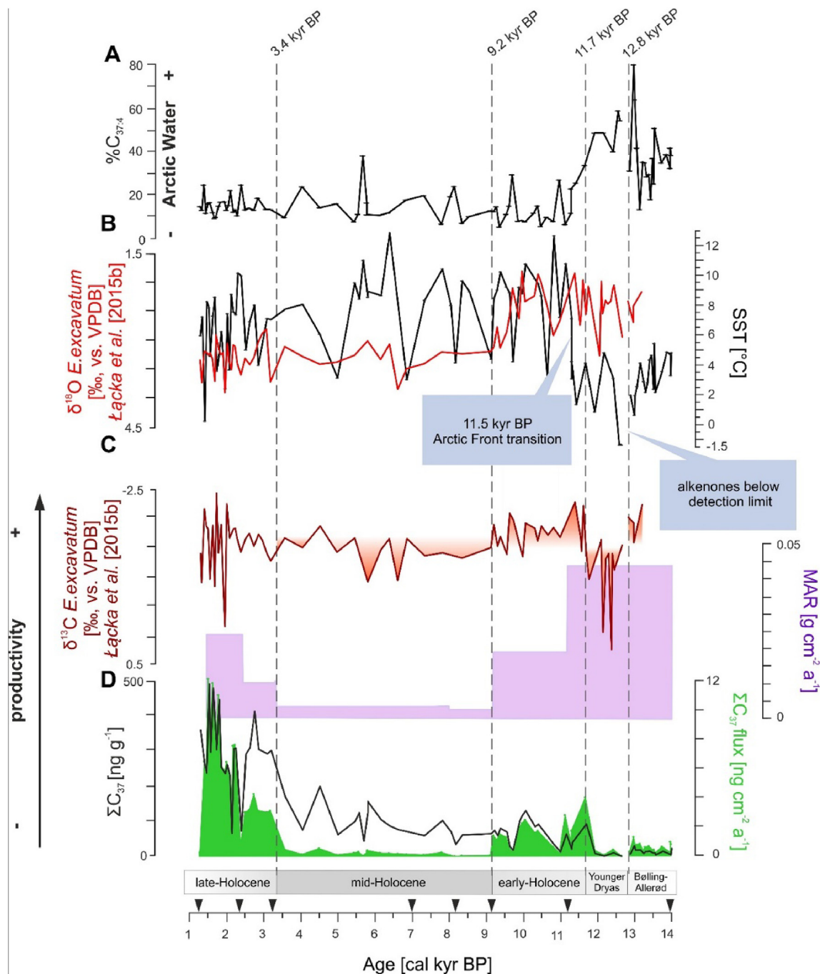
Fig. 3. Proxy records from core JM09-020 GCA: A) \%C_{37:4} ; B) U^{K}_{37} -based sea surface temperatures (SSTs; right scale) and stable oxygen isotope data (red line; left scale; Łącka et al., 2015b); C) stable carbon isotope data (burgundy line; left scale; Łącka et al., 2015b) and mass accumulation rates ( g\ cm^{-2}\ a^{-1} ; violet shading; right scale; Łącka et al., 2015b); D) total alkenone concentrations ( \Sigma C_{37} ; ng\ g^{-1} ; black line; left scale) and total alkenone flux ( ng\ cm^{-2}\ a^{-1} ; green shading; right scale). The black triangles on the x axis denote the AMS ^{14}C converted to calibrated radiocarbon ages (after Łącka et al., 2015b). The Arctic Front transition at 11,500 cal yr BP is marked. (For interpretation of the references to color in this figure legend, the reader is referred to the Web version of this article.)
